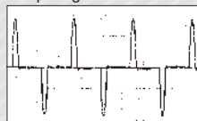
Current waveform from an inverter (primary side)
